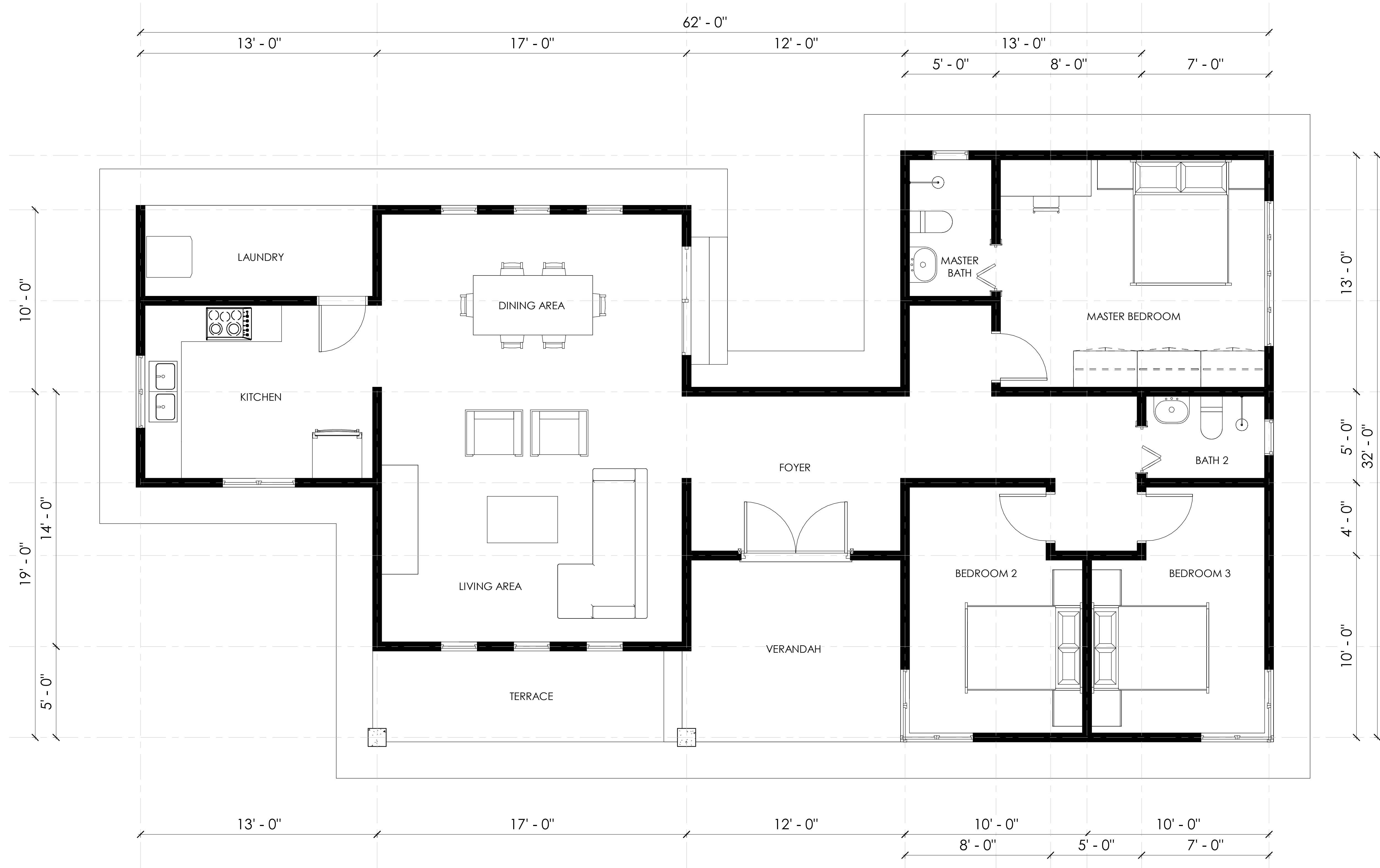
FLOOR PLAN
